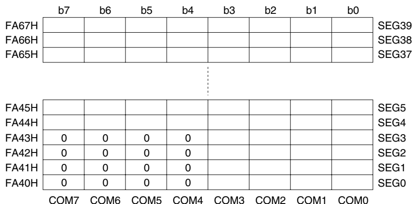
Figure 18-15. Relationship between LCD Display Data Memory Contents and Segment/Common Outputs
