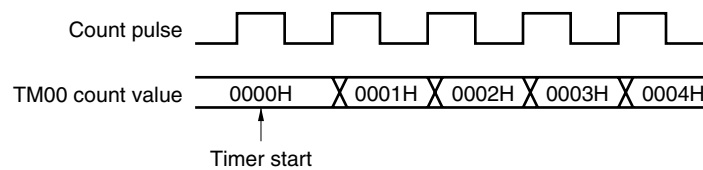
Figure 6-59. Start Timing of TM00 Count
