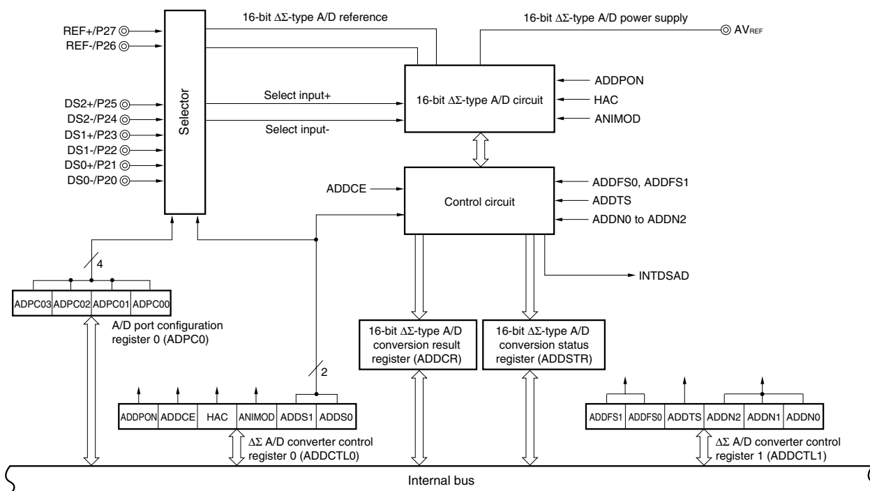
Figure 13-1. Block Diagram of 16-Bit ΔΣ-Type A/D Converter
