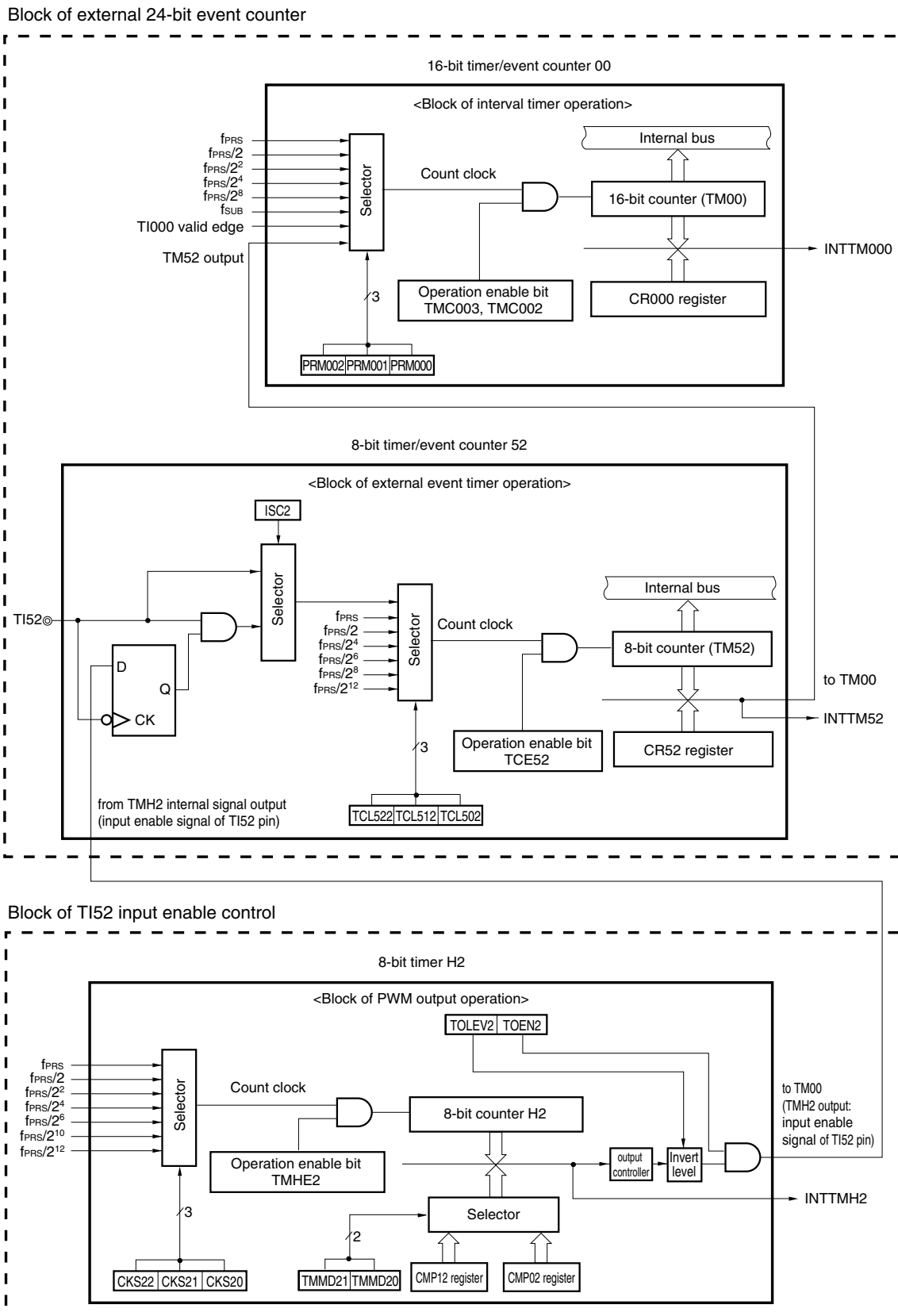
Figure 6-54. Configuration Diagram of External 24-bit Event Counter
