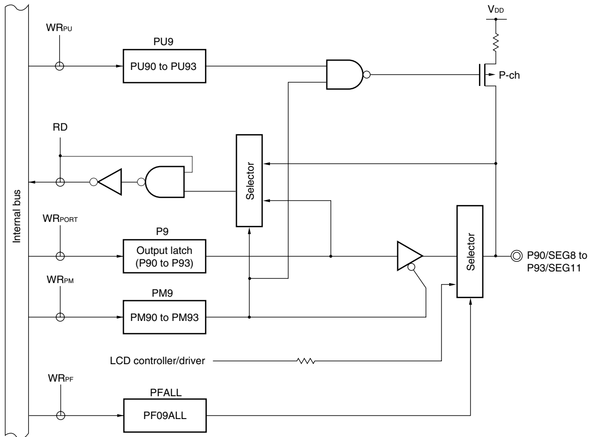
Figure 4-15. Block Diagram of P90 to P93
