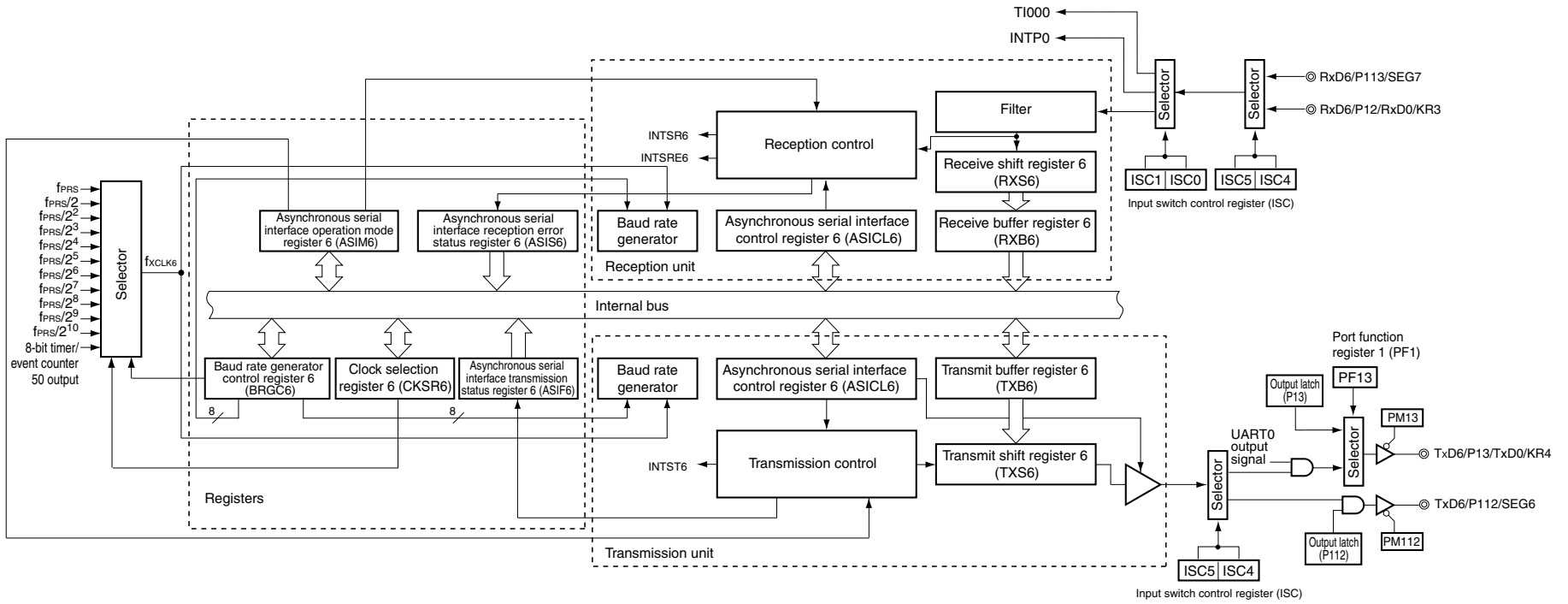
(a) 78K0/LC3
