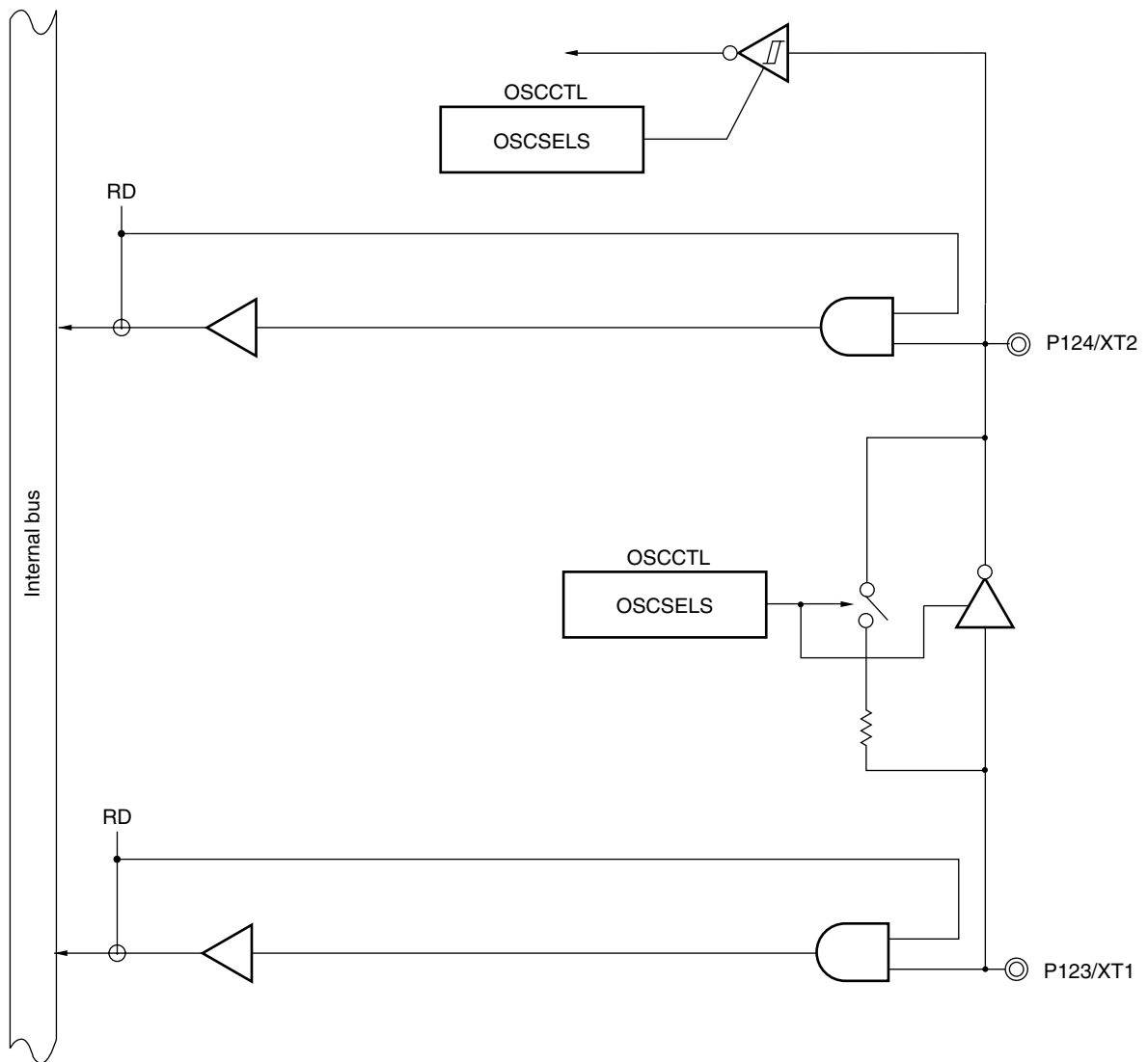
Figure 4-22. Block Diagram of P123 and P124
