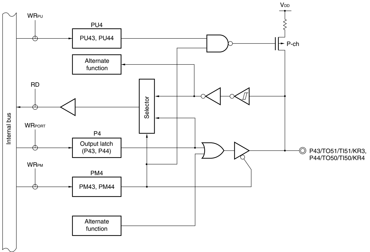
Figure 4-13. Block Diagram of P43 and P44
