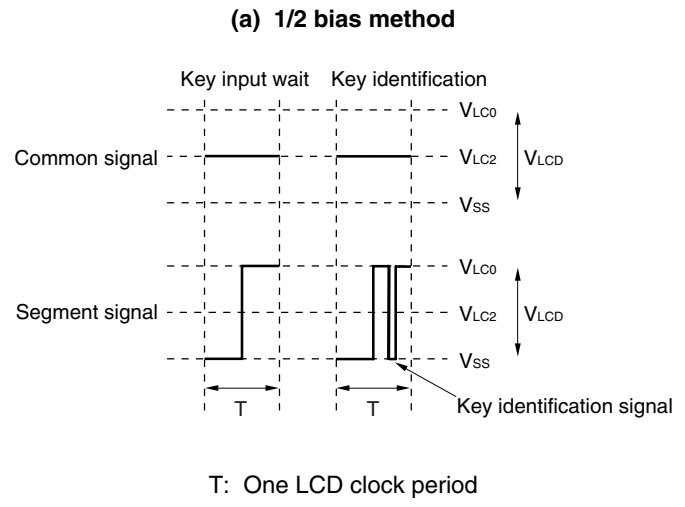
Figure 18-19 Voltages and Phases of Common and Segment Signals
