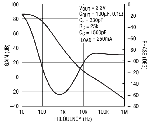
Figure 11. Overall Loop Response
