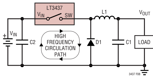
Figure 8. High Speed Switching Path
